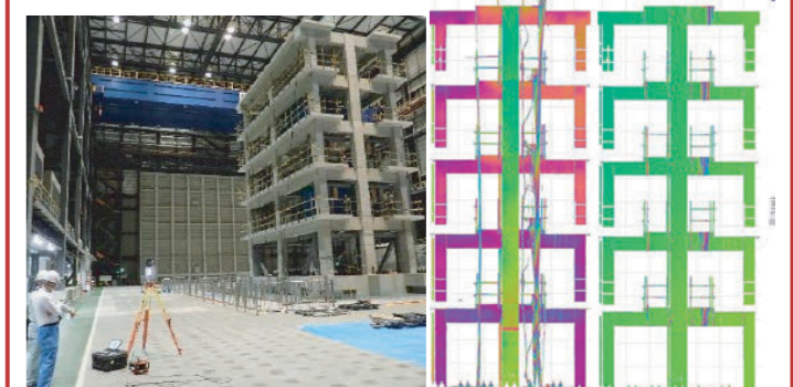
レーザースキャナーを用いた被災建物調査手法の開発 Development of a method for surveying damaged buildings using a laser scanner
