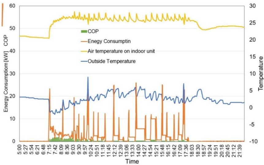
Figure 2.4.2-3. Defrost during heating operation
